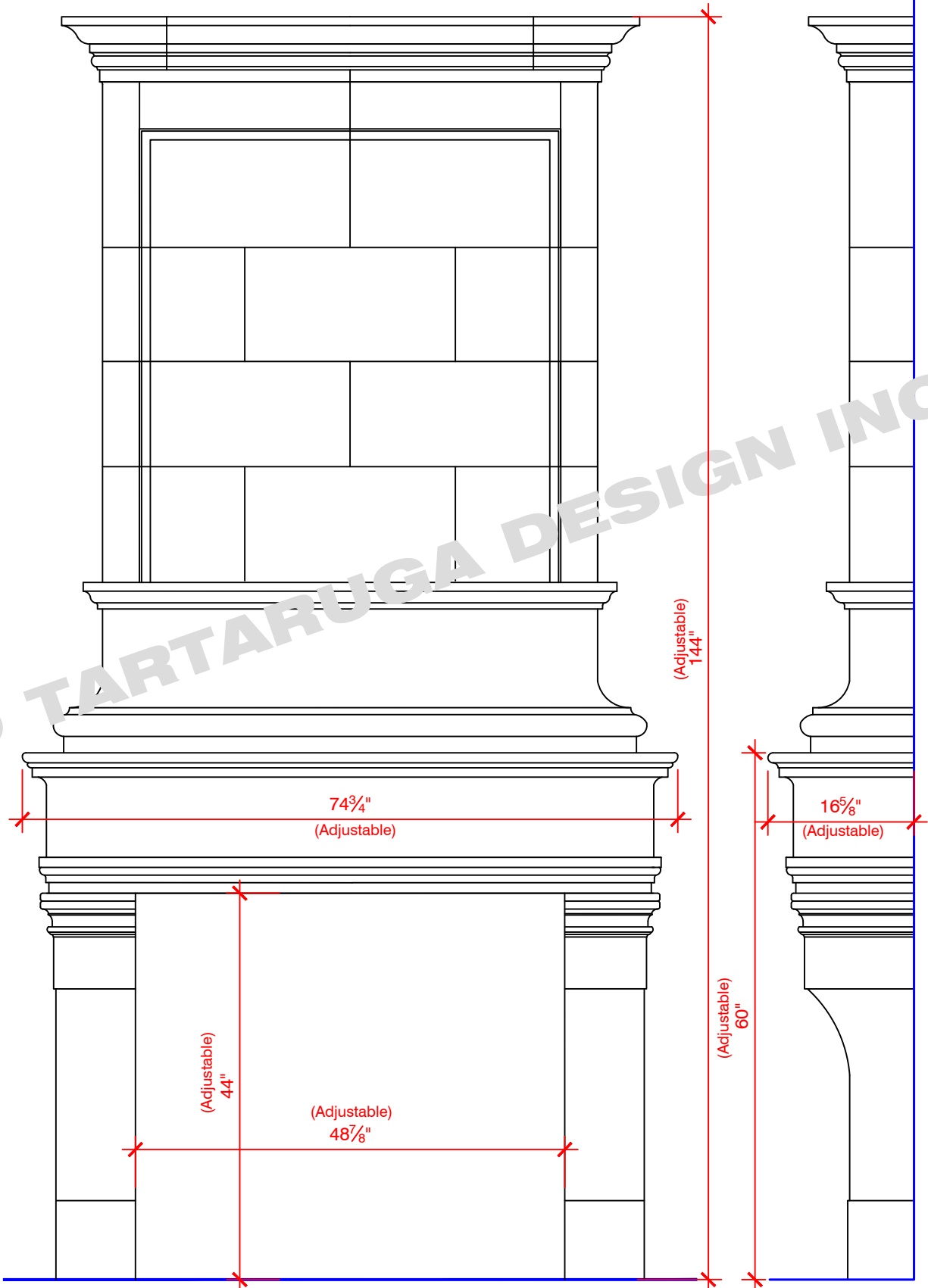
FRONT VIEW
