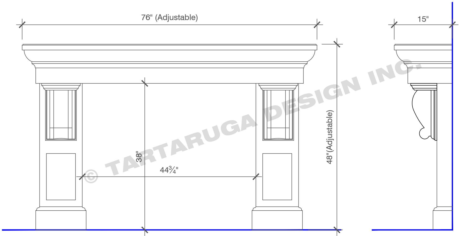
FRONT VIEW
