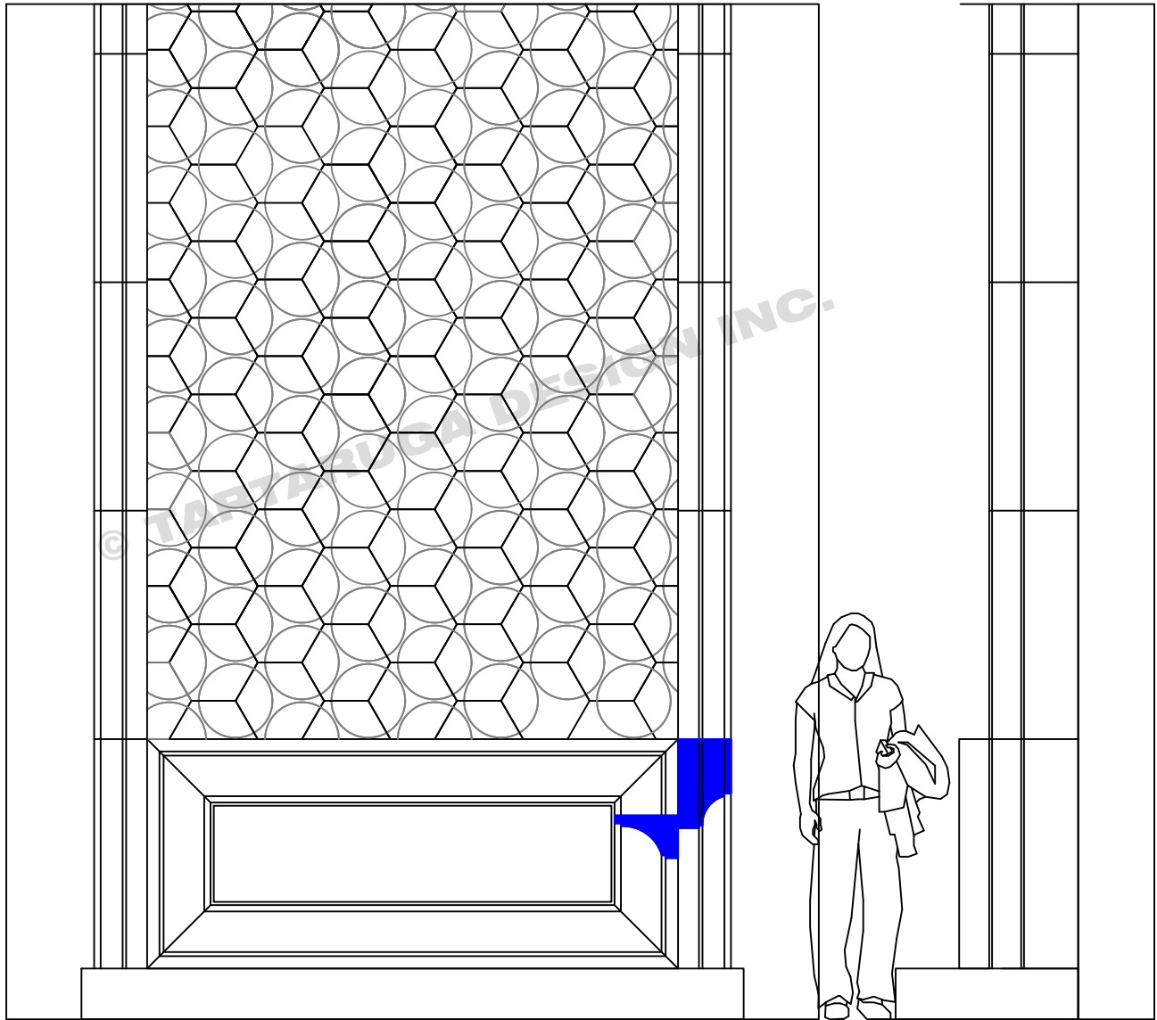
FRONT ELEVATION
