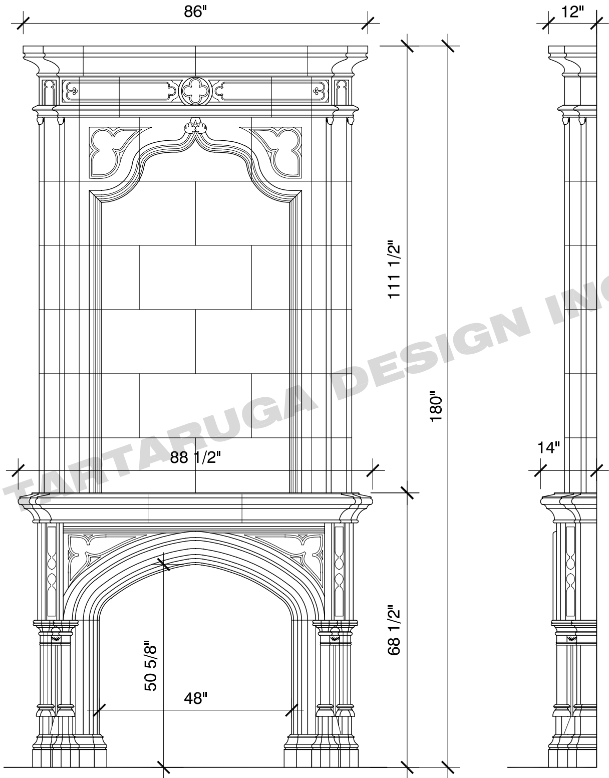
FRONT VIEW
