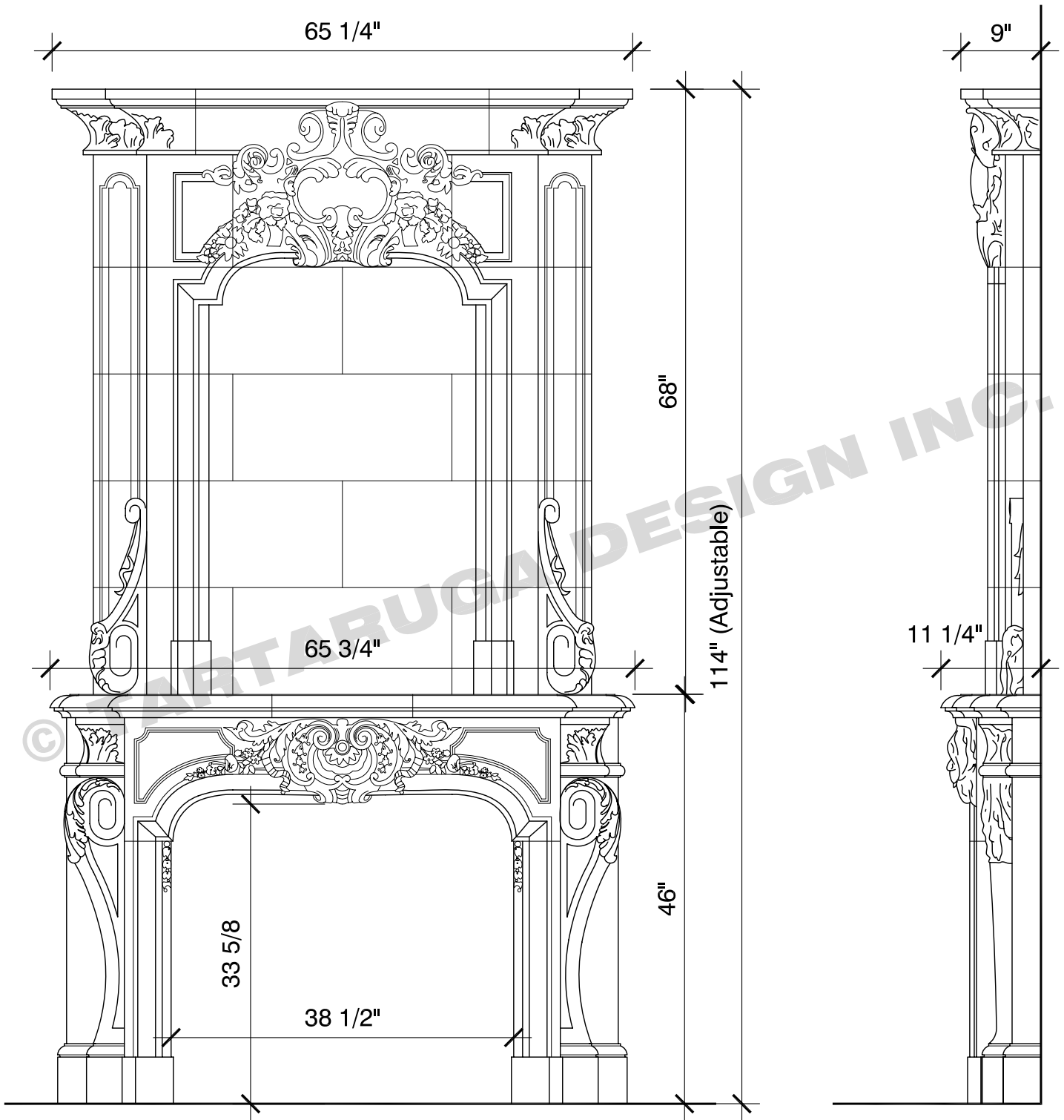
FRONT VIEW
