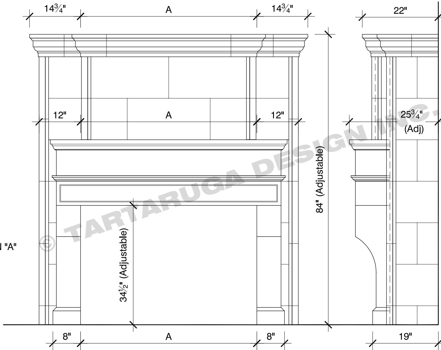
FRONT VIEW
