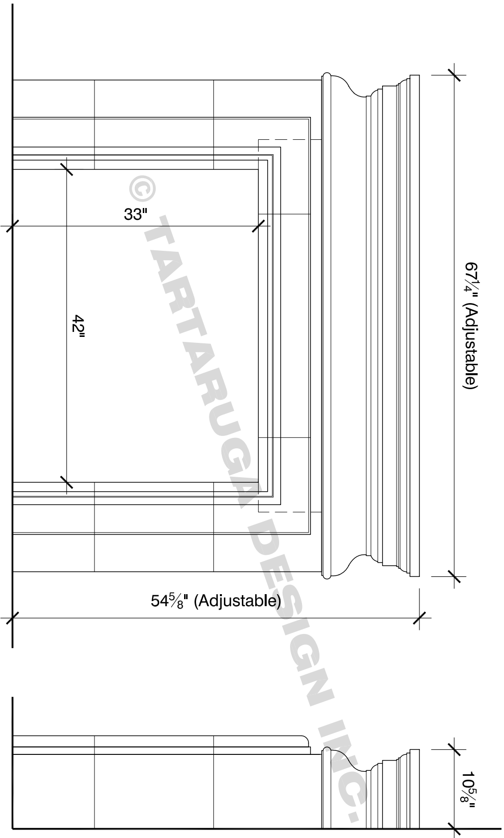
FRONT VIEW
