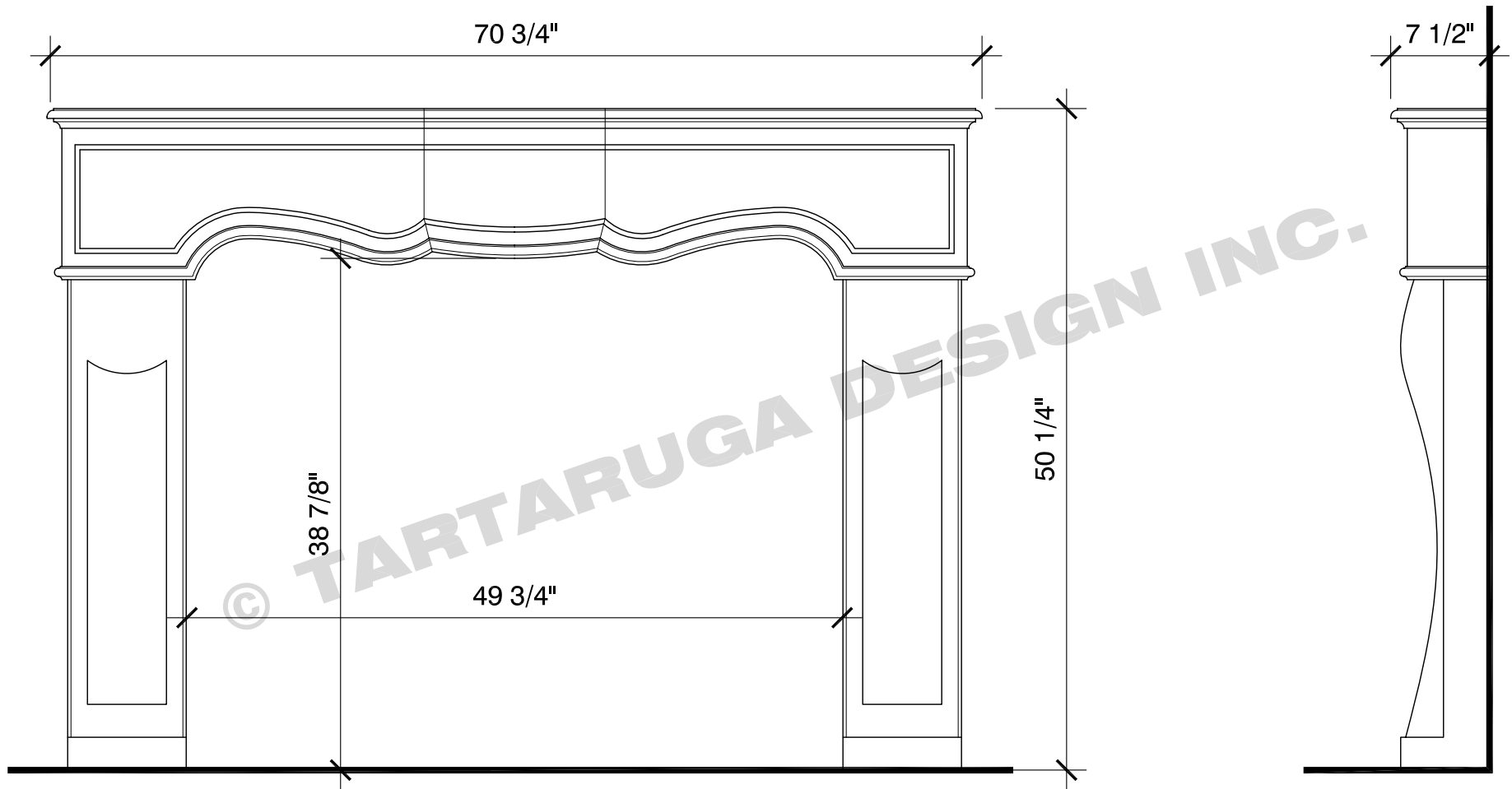
FRONT VIEW
