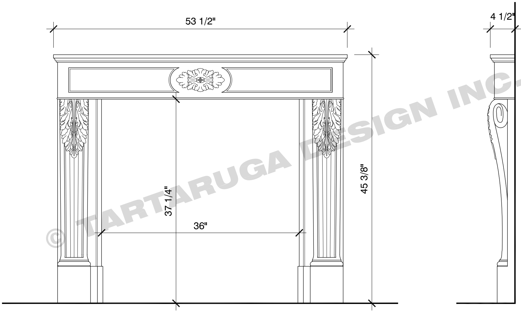
FRONT VIEW
