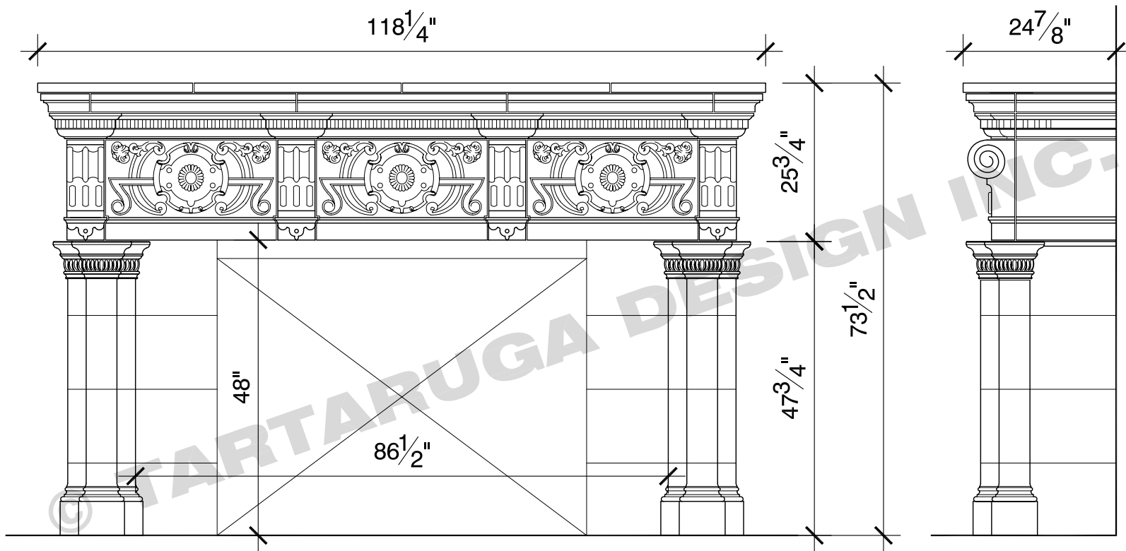
FRONT VIEW
