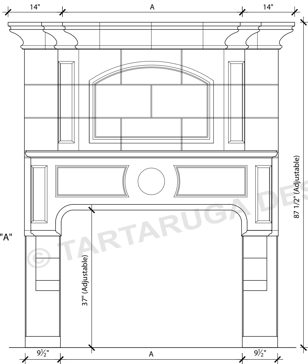
FRONT VIEW
