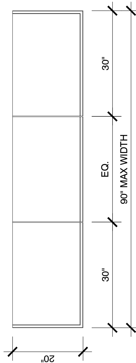
HEARTH PLAN 3/4" = 1'-0" SCALE
