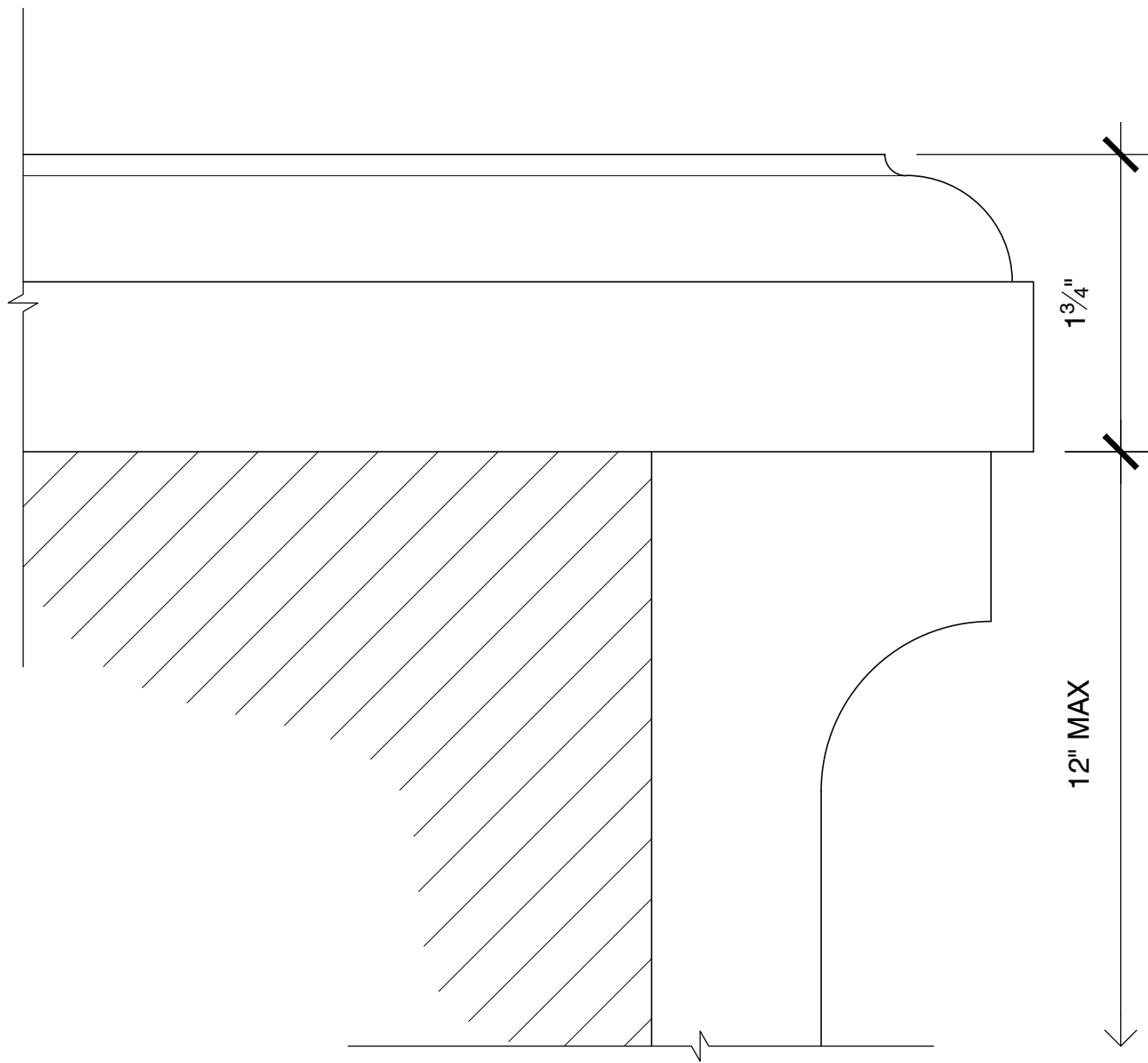
PROFILE SECTION - FULL SCALE
