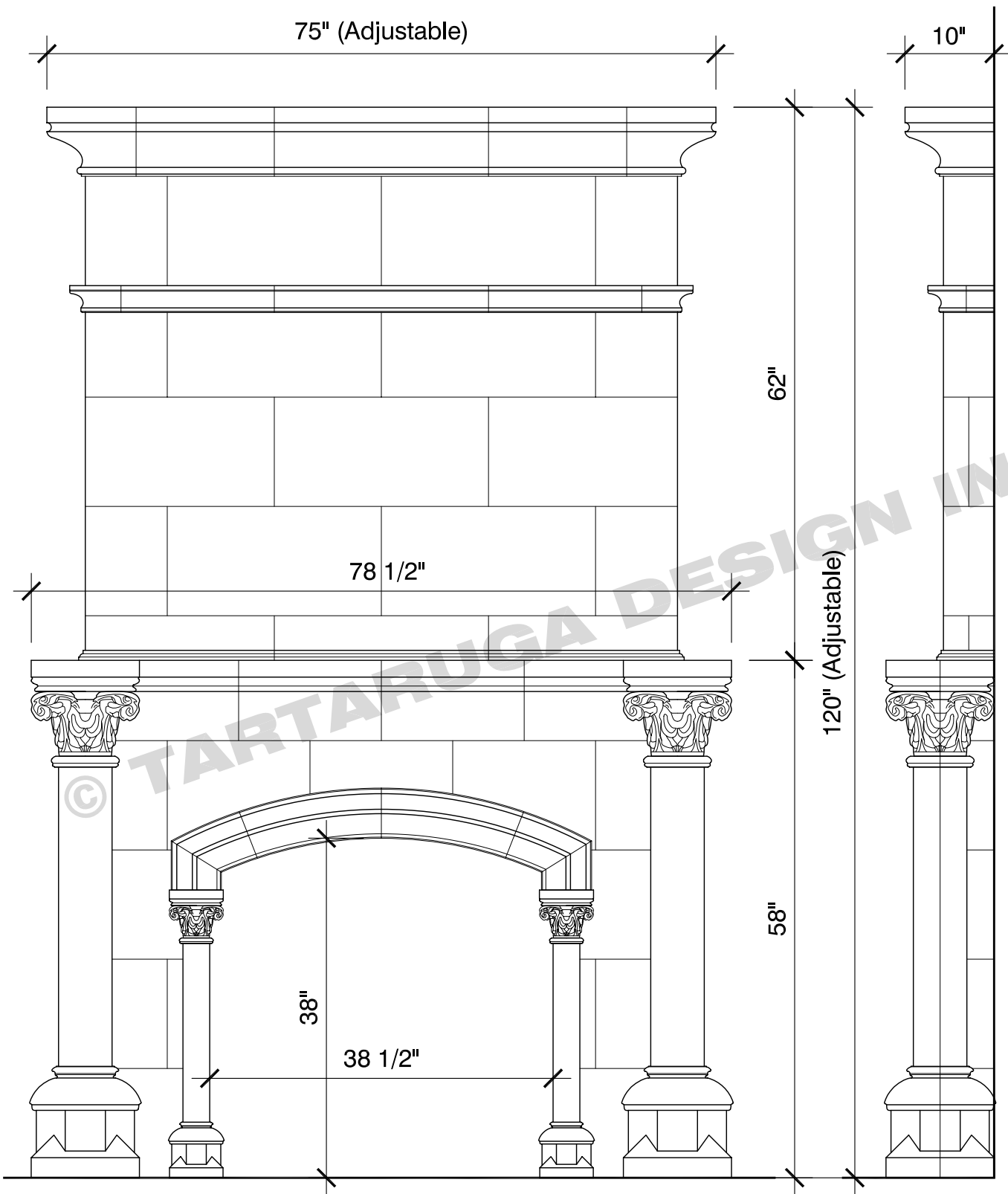
FRONT VIEW
