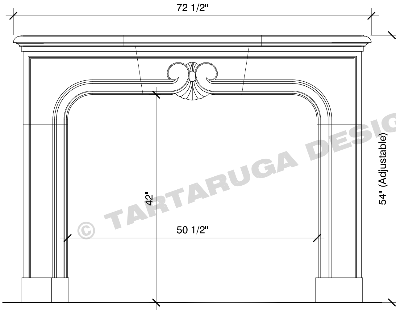
FRONT VIEW
