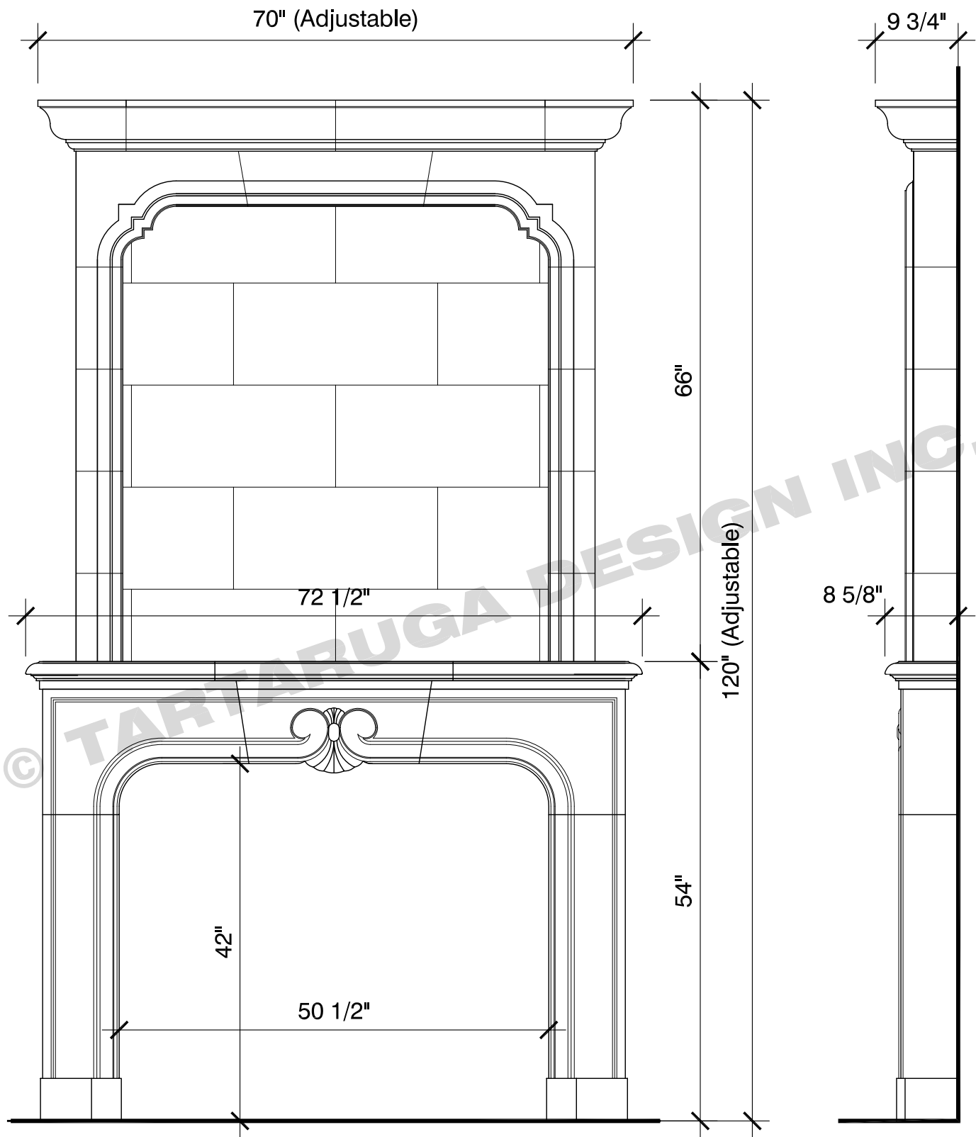
FRONT VIEW
