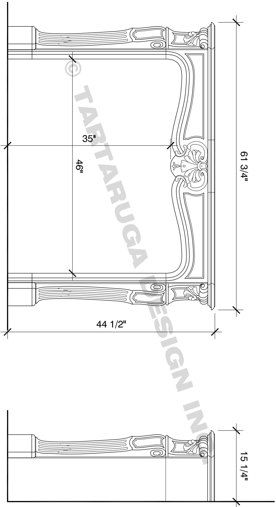
FRONT VIEW
