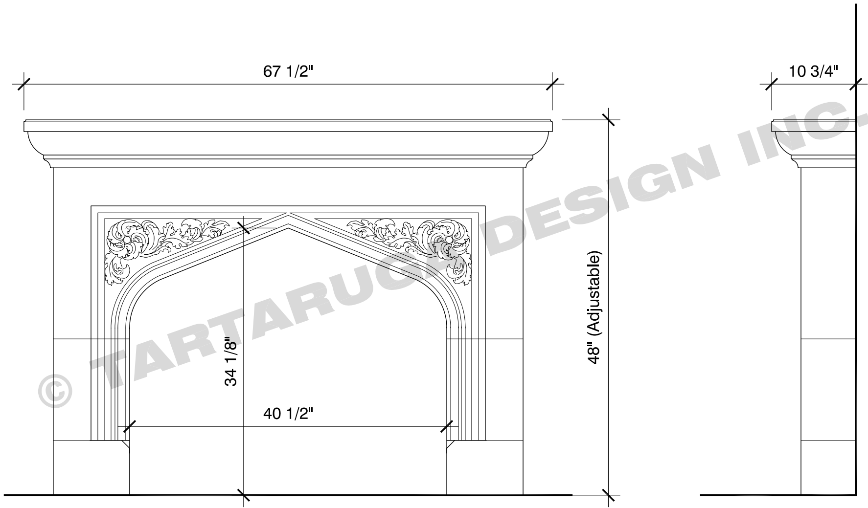
FRONT VIEW
