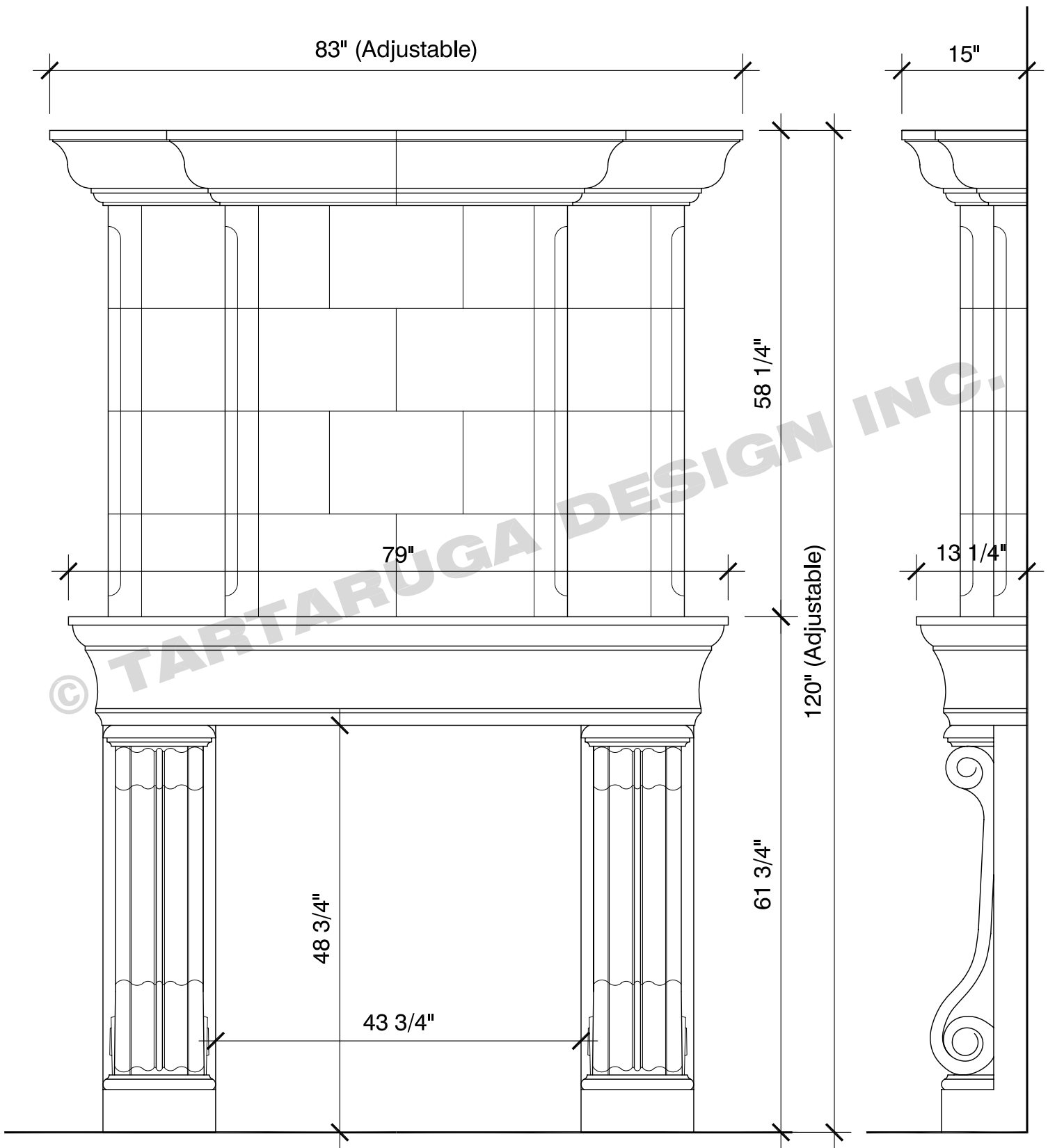
FRONT VIEW
