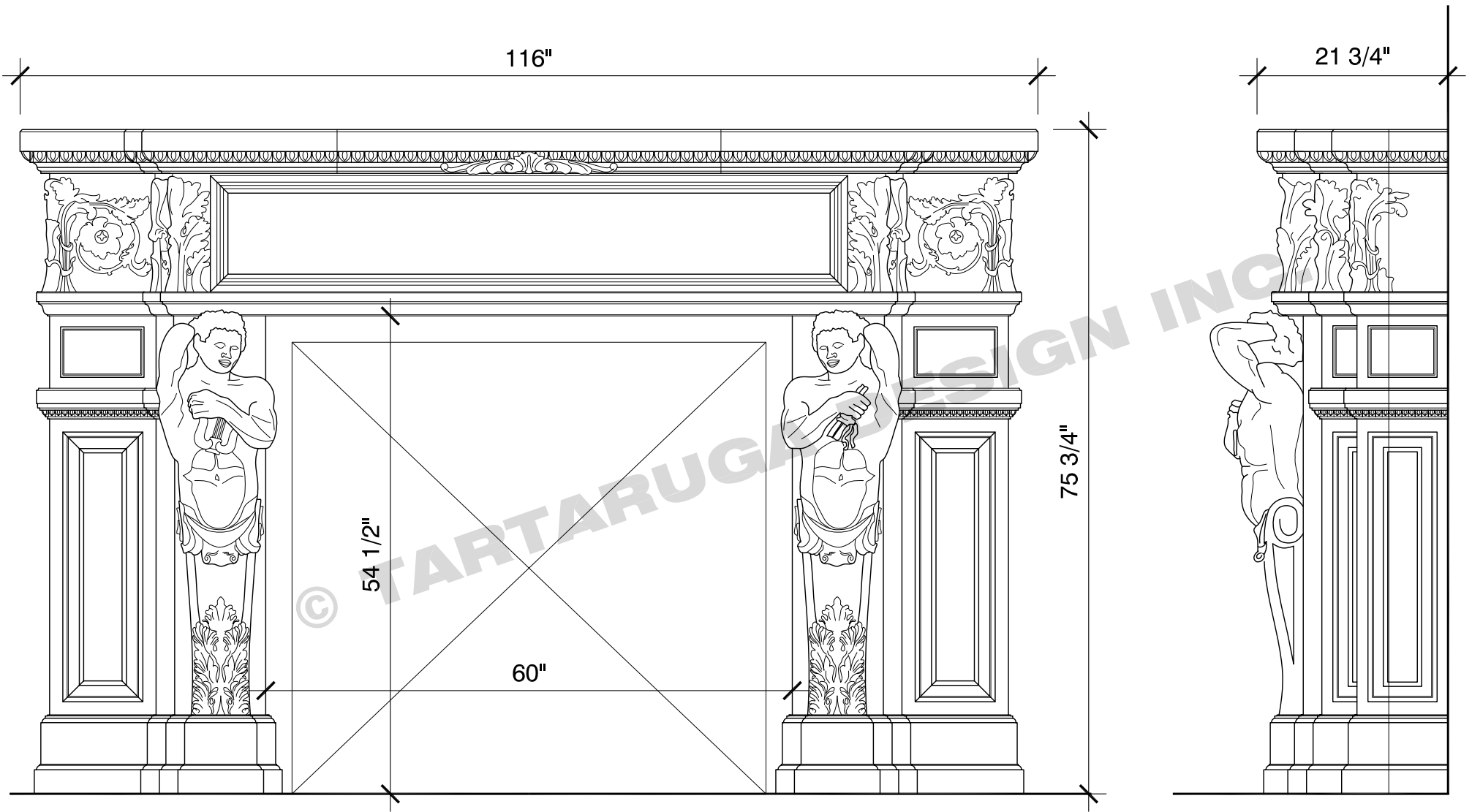
FRONT VIEW
