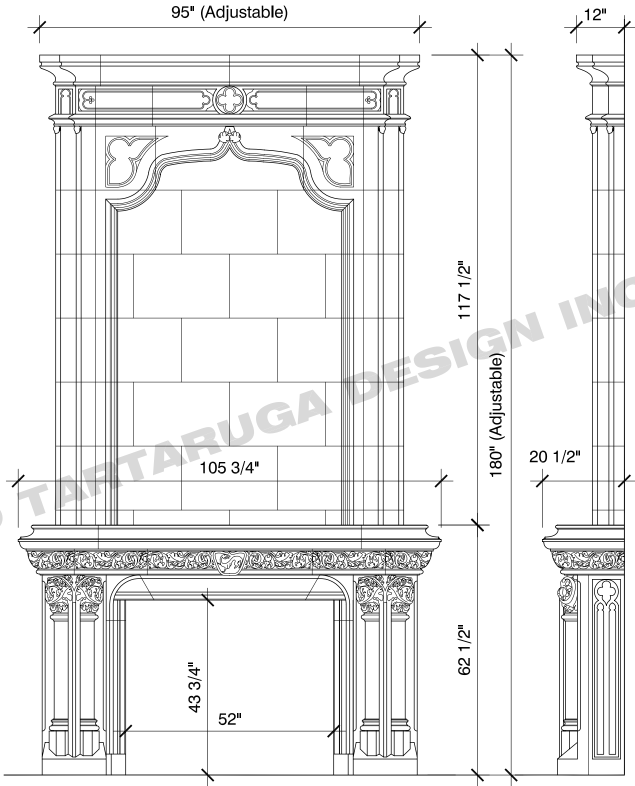
FRONT VIEW
