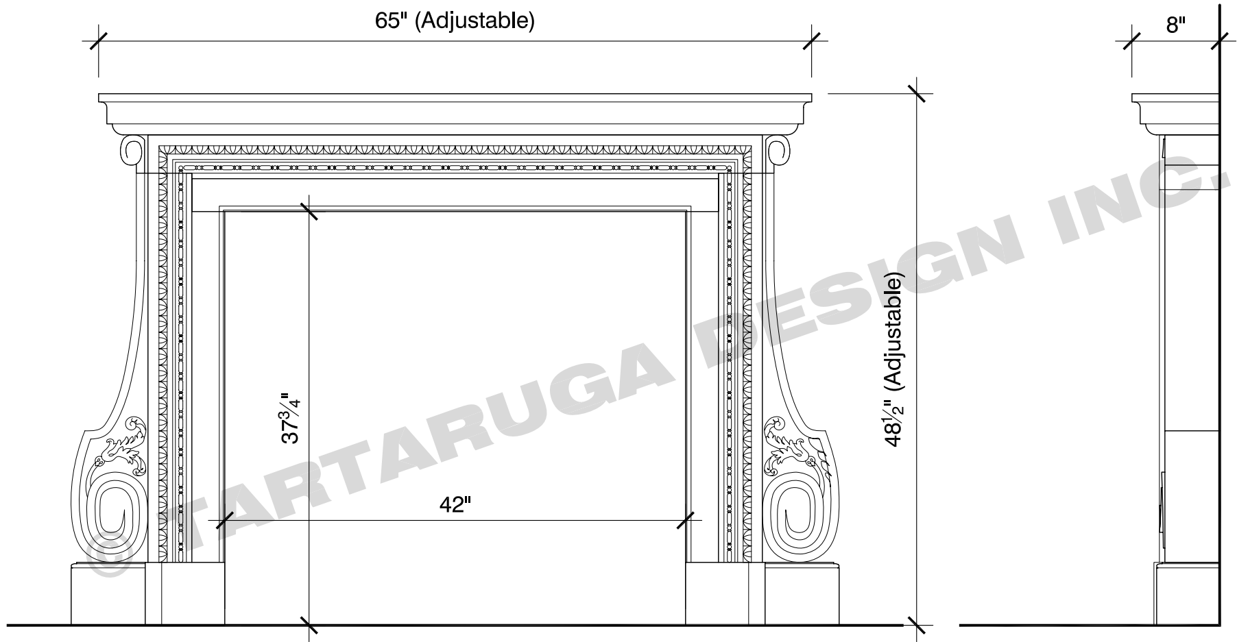
FRONT VIEW
