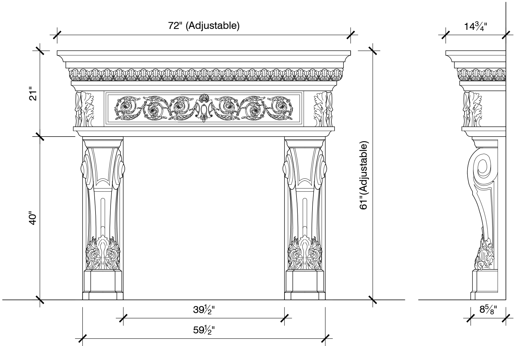
SIDE VIEW
